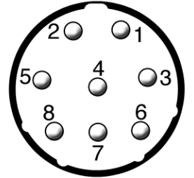
AMP Connector and pins (Male connector) View from back of plug
