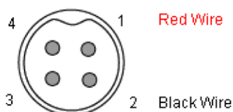
Front view of SmartPak power cable 1-1701.260
