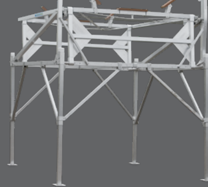
DEEP-WATER LEVELING LEGS WITH BRACING
