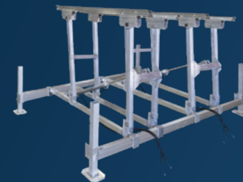
PWC LIFTS 5,000 Double PWC Lift (Two hydraulic cylinders)
