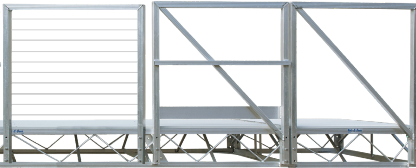
TRUSS HANDRAIL SHOWN WITH MIDRAIL AND KICKRAIL OPTION
