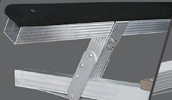
ALUMINUM V-BUNK FOR INBOARD
