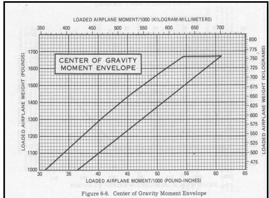
Figure 6-8. Center of Gravity Moment Envelope
