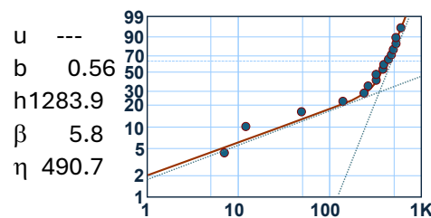
Figure 13: YBath™ Advanced Mixture Models (Page 1 of 2) From Carl Tarum.
