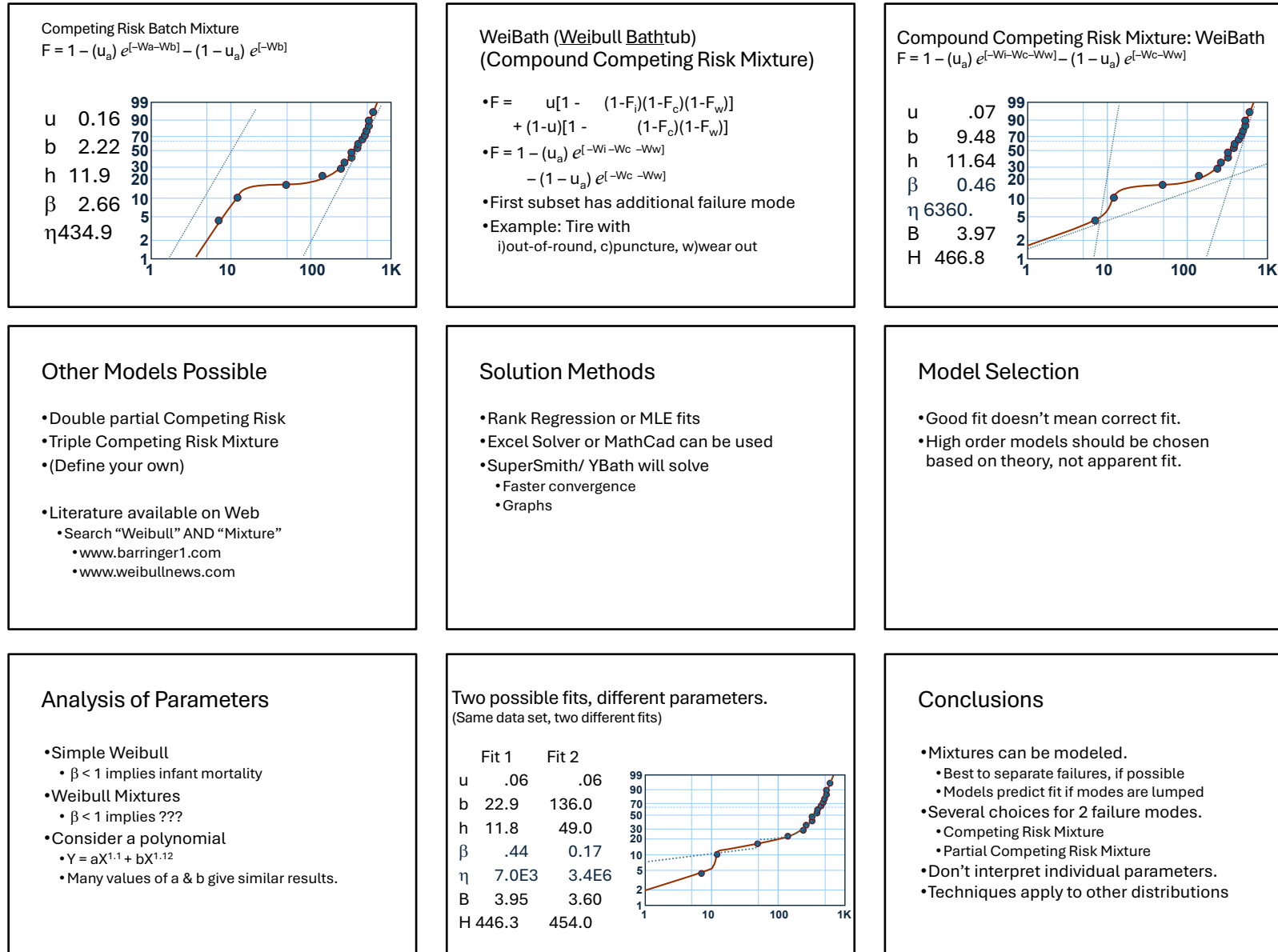
Figure 14: YBath™ Advanced Mixture Models (Page 2 of 2) from Carl Tarum.
