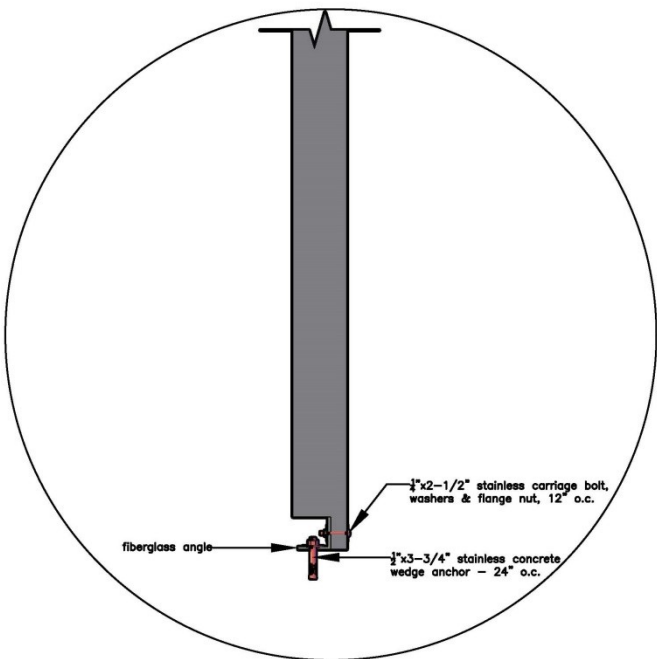
Fiberglass angle
