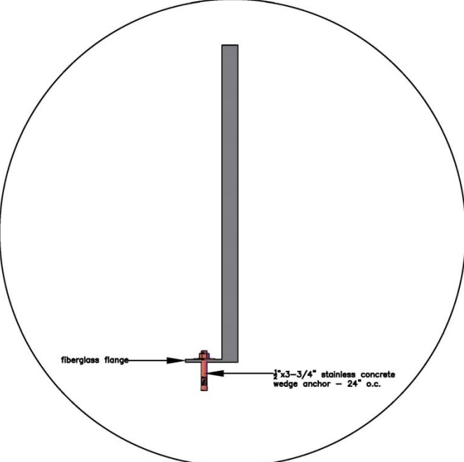
Fiberglass flange
