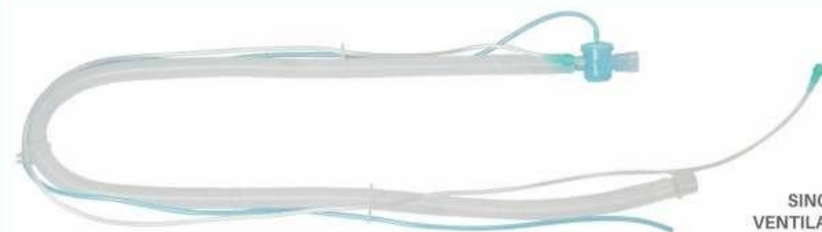
CARAT 2 PRO VENTILATOR CIRCUIT MK 6000
