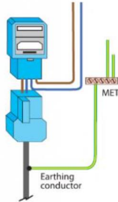
Earthing System TN-S Z_e 0.24 \Omega
