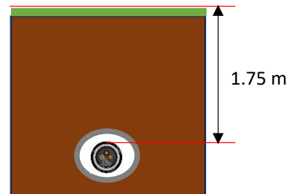
Cable Installation Depth. 1.75 metres
