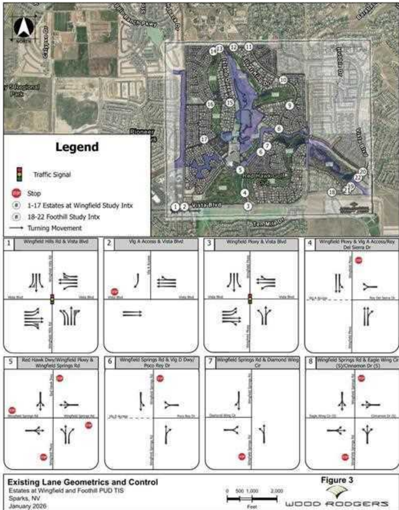
Figure 3. Existing Conditions Lane Geometrics and Control
