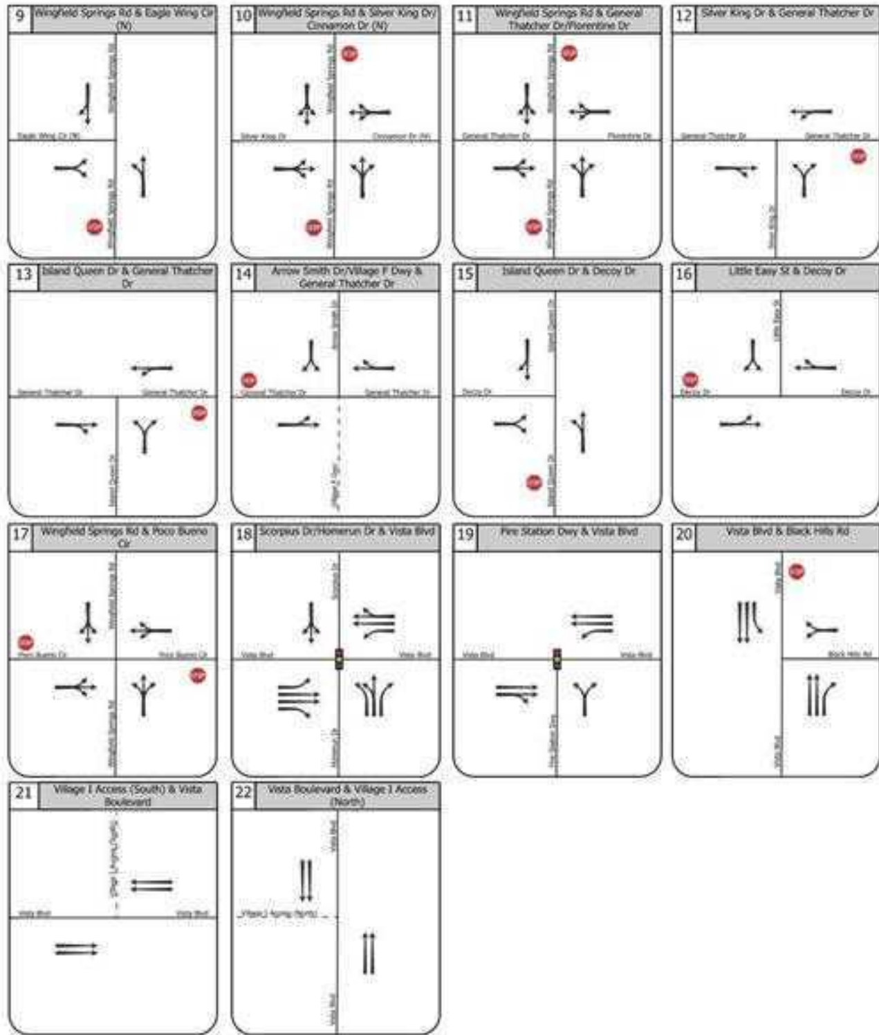
Figure 3. Existing Conditions Lane Geometrics and Control
