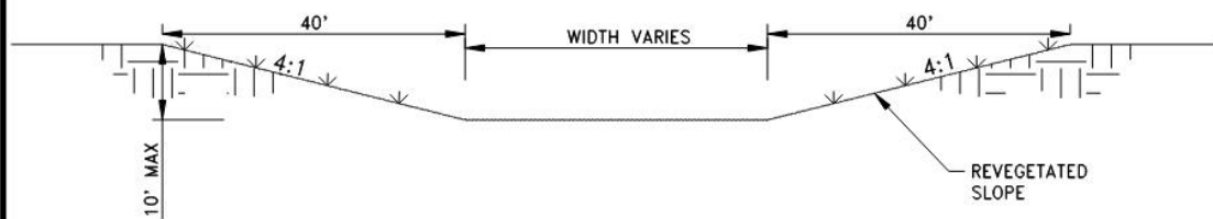
4:1 SIDE SLOPE REVEGETATED CHANNEL
