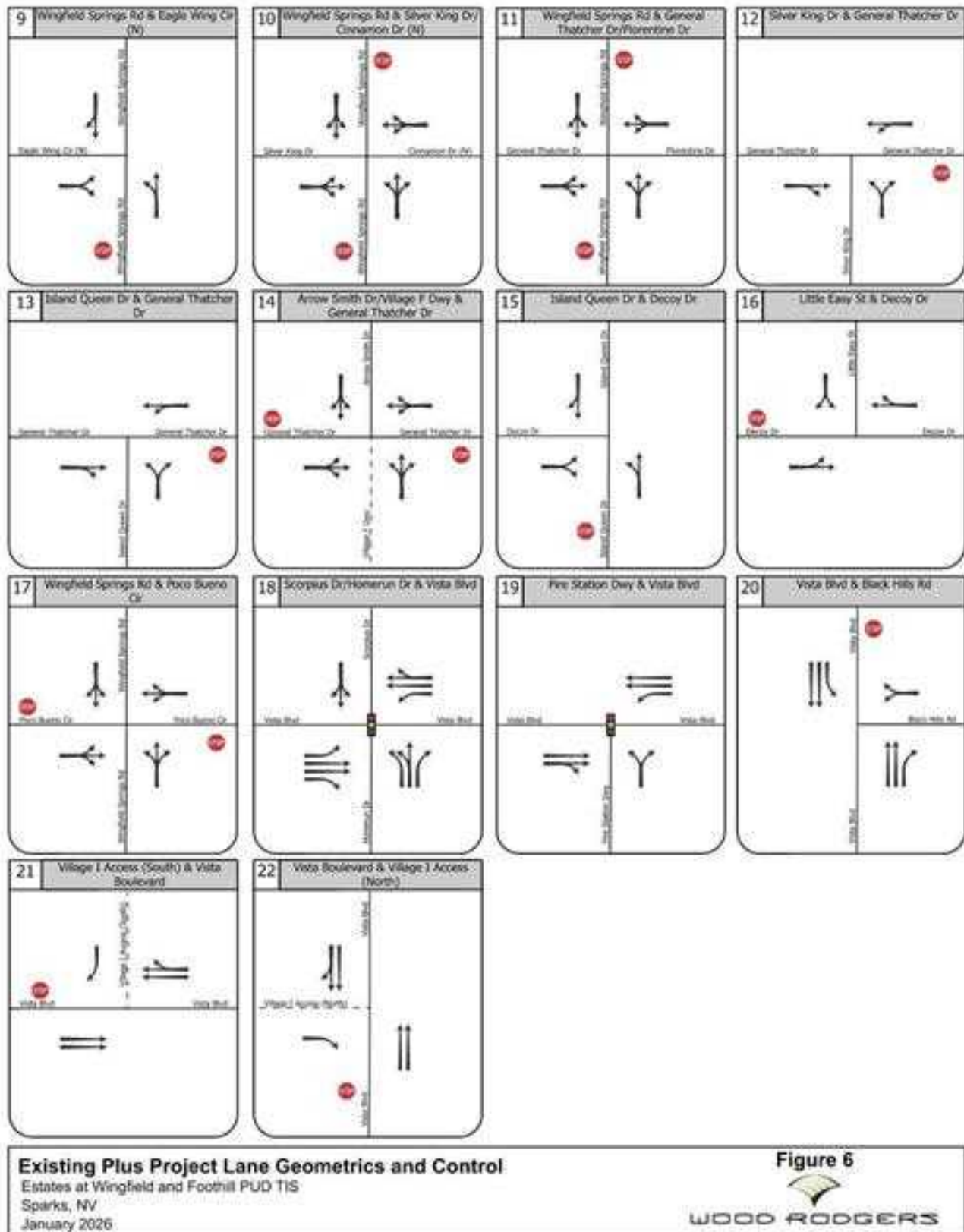
Figure 6. Existing Plus Project Lane Geometrics and Control
