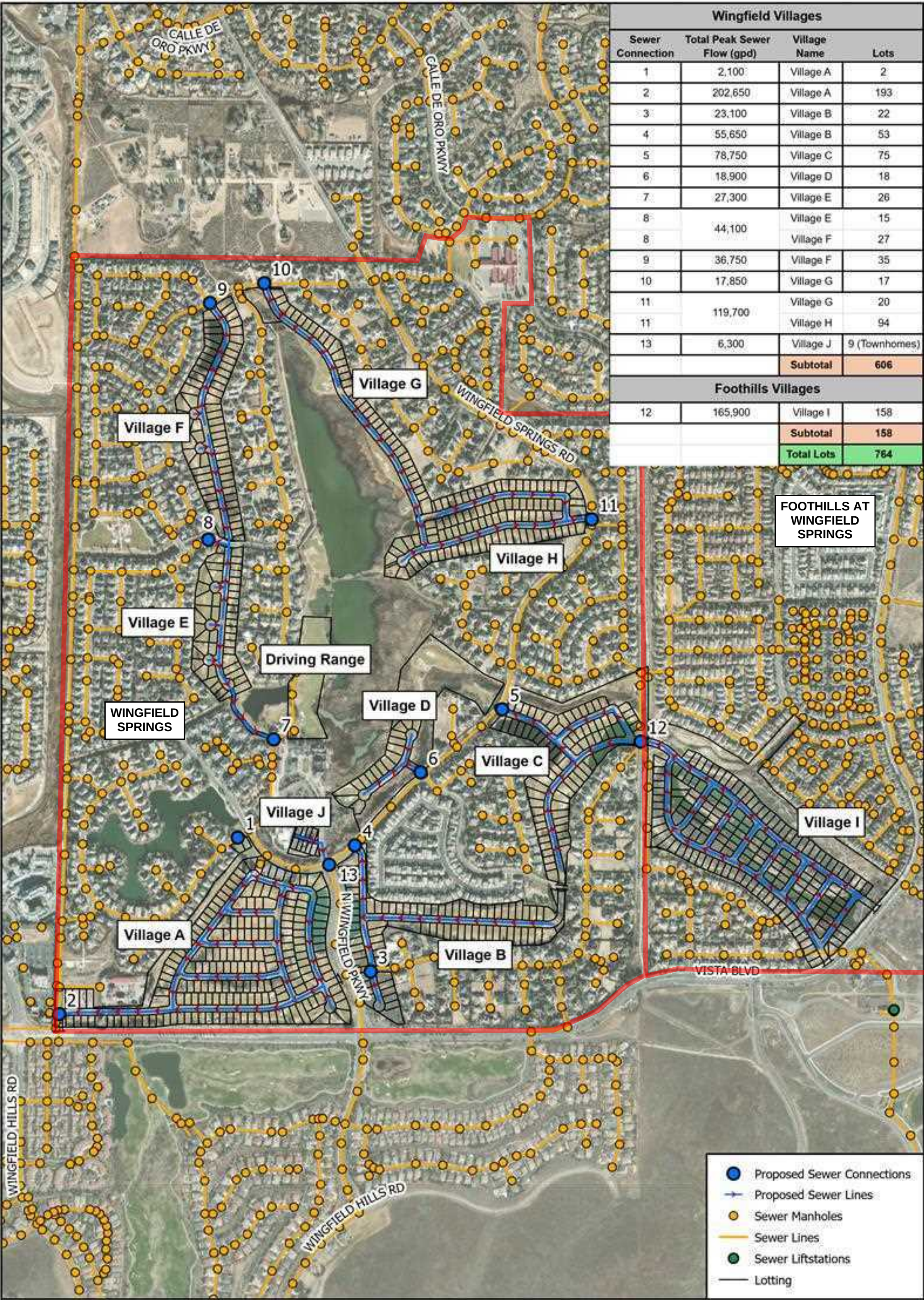
PRELIMINARY SEWER SHED MAP WINGFIELD SPRINGS AND FOOTHILLS AT WINGFIELD SPRINGS SPARKS, NV JANUARY 2026 NOTES: Sewer flow based on 350 gpd / capita, 3 capita / unit for SFR, and 2 capita / unit for townhomes
