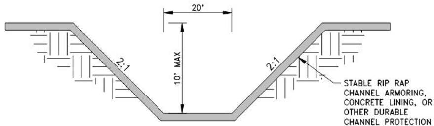
2:1 SIDE SLOPE ARMORED CHANNEL
