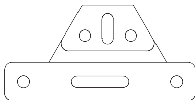
Left PEBA hinge x1
