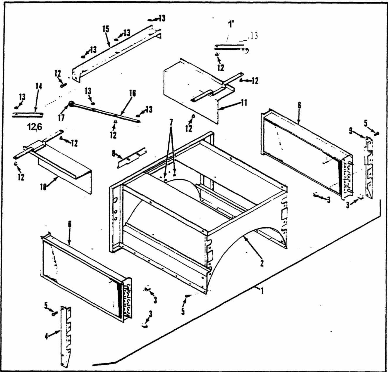
Figun1 6-4. Manual Damper Steam Heating Unit
