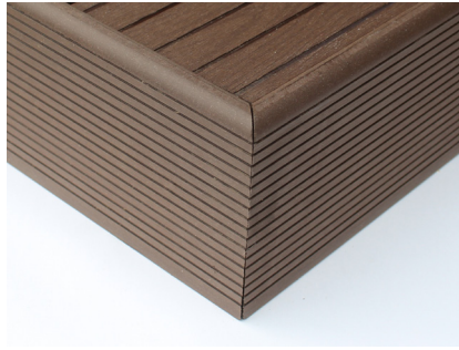
Two configurations with Bullnose Boards used as edging
