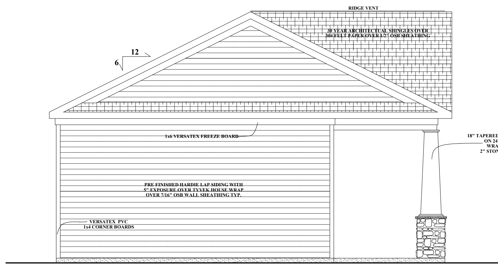
LEFT ELEVATION
