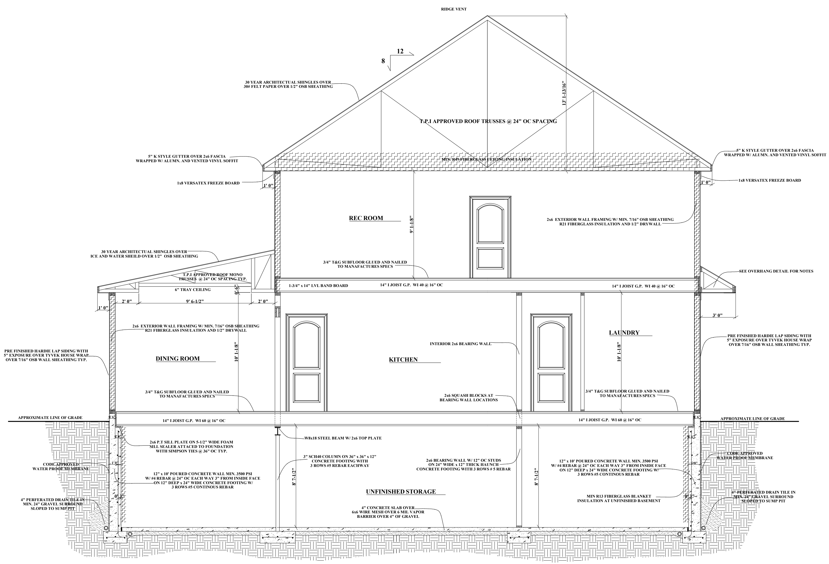
SECTION 1-B
