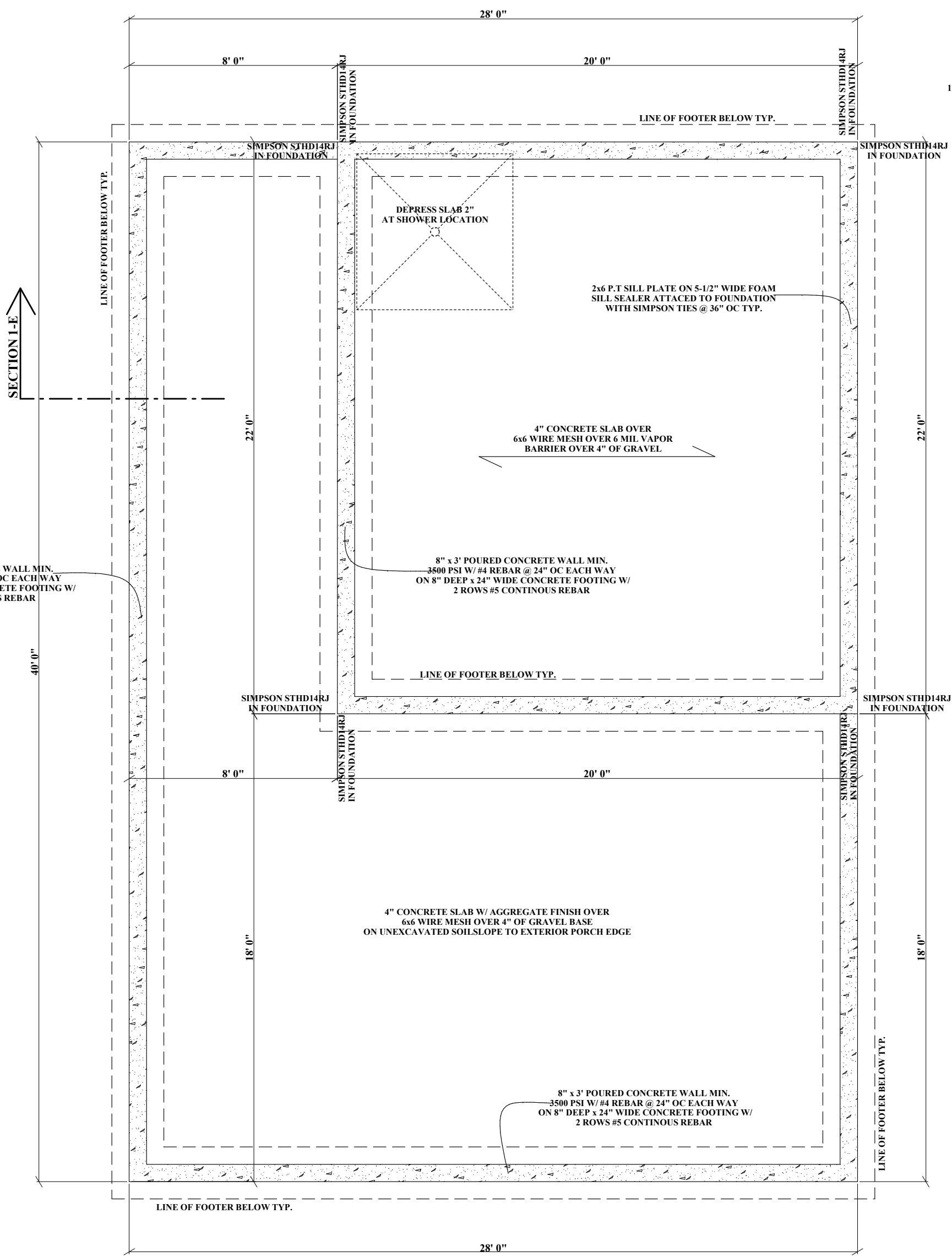
FOUNDATION PLAN
