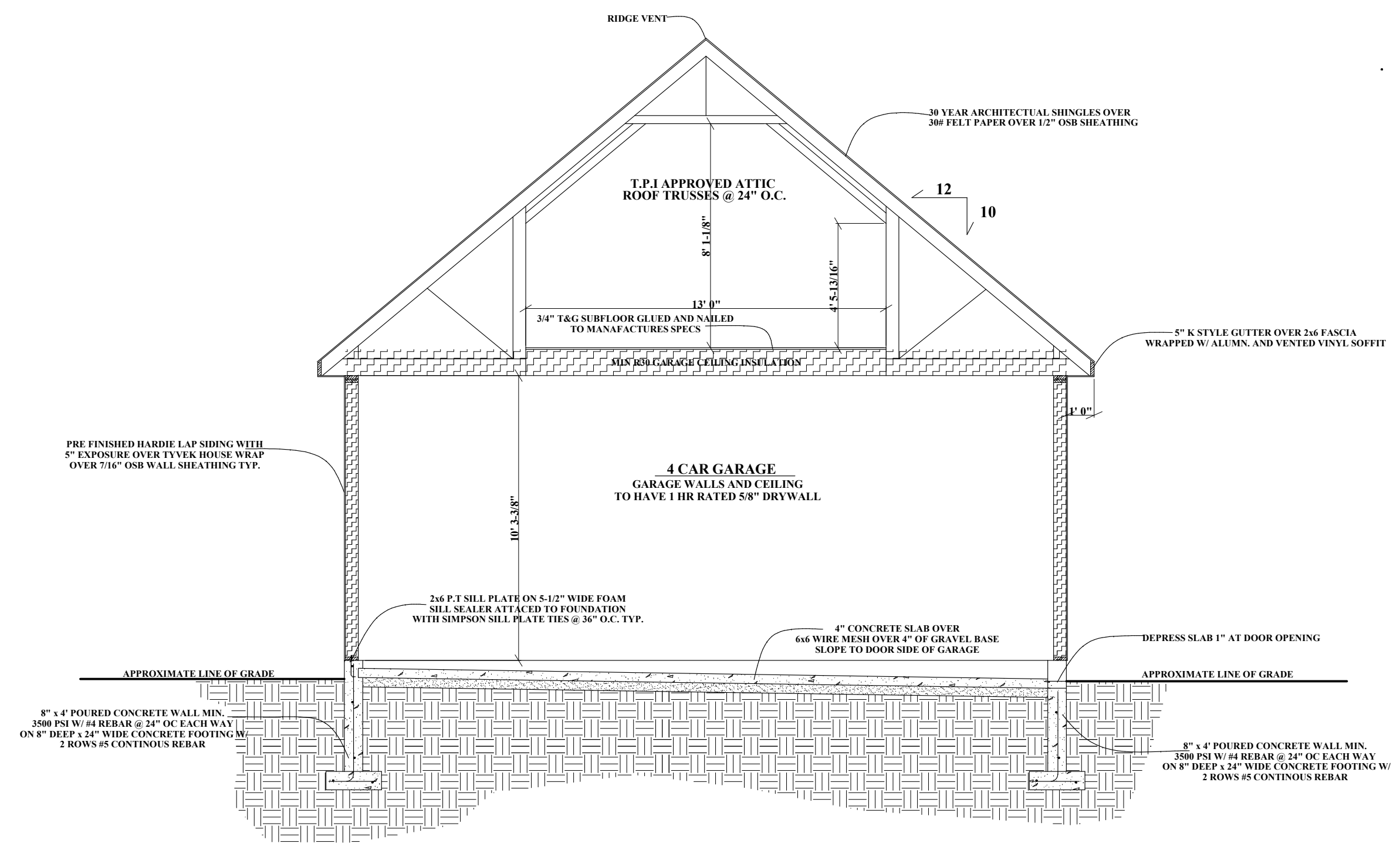
SECTION 1-C
