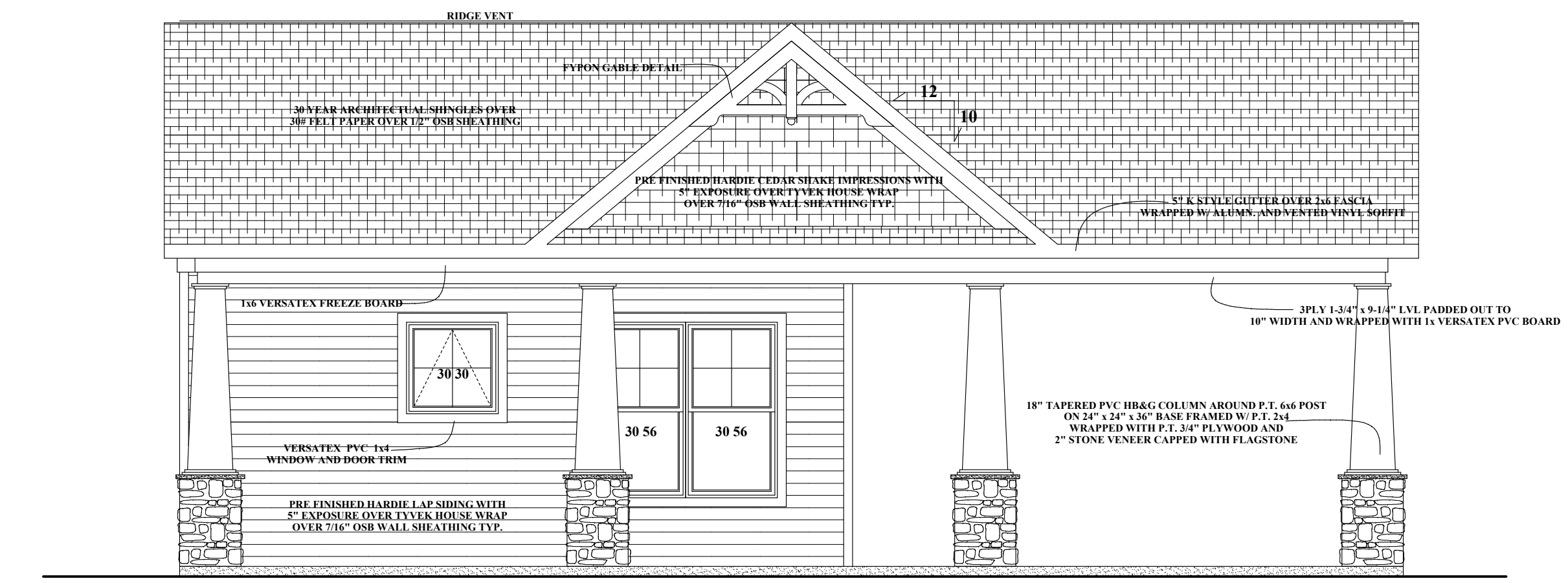
FRONT ELEVATION
