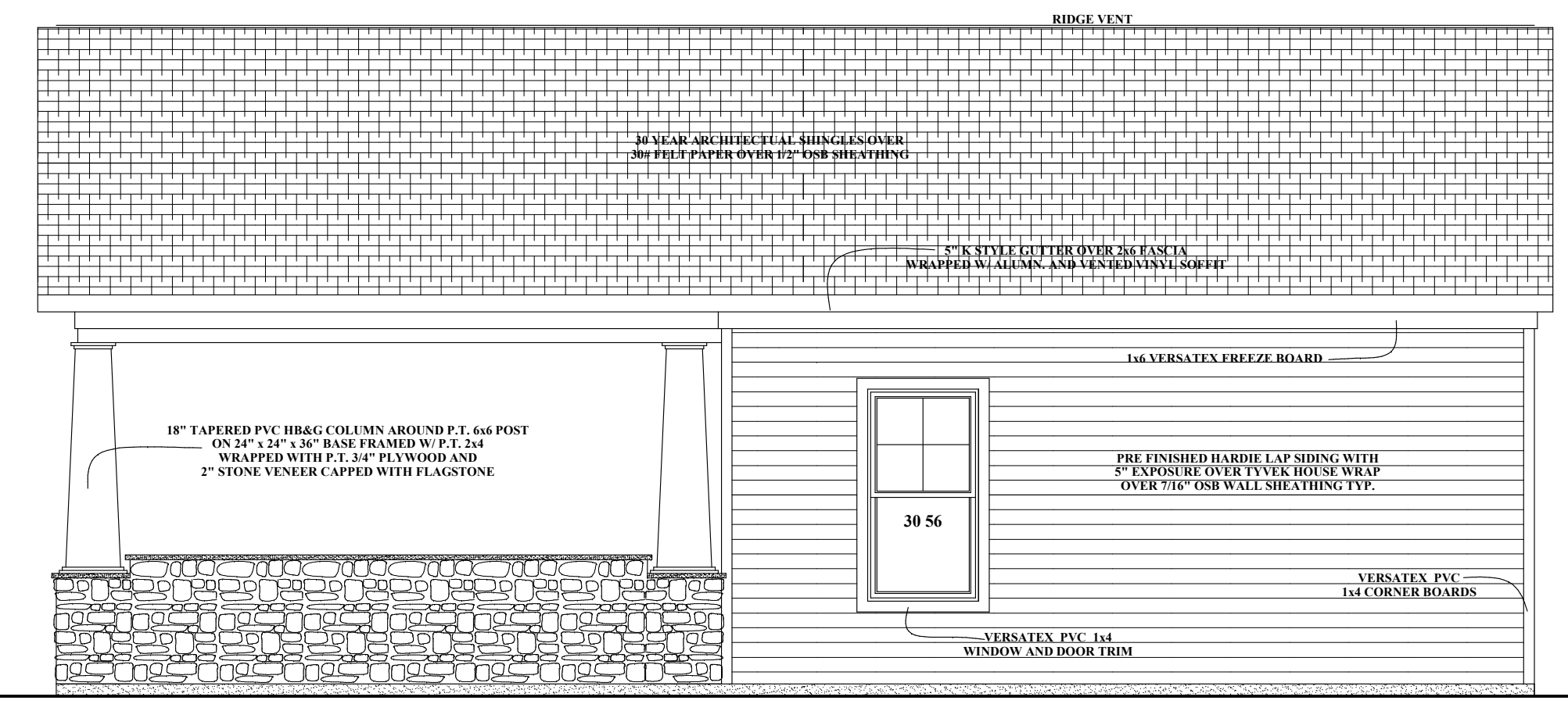
REAR ELEVATION
