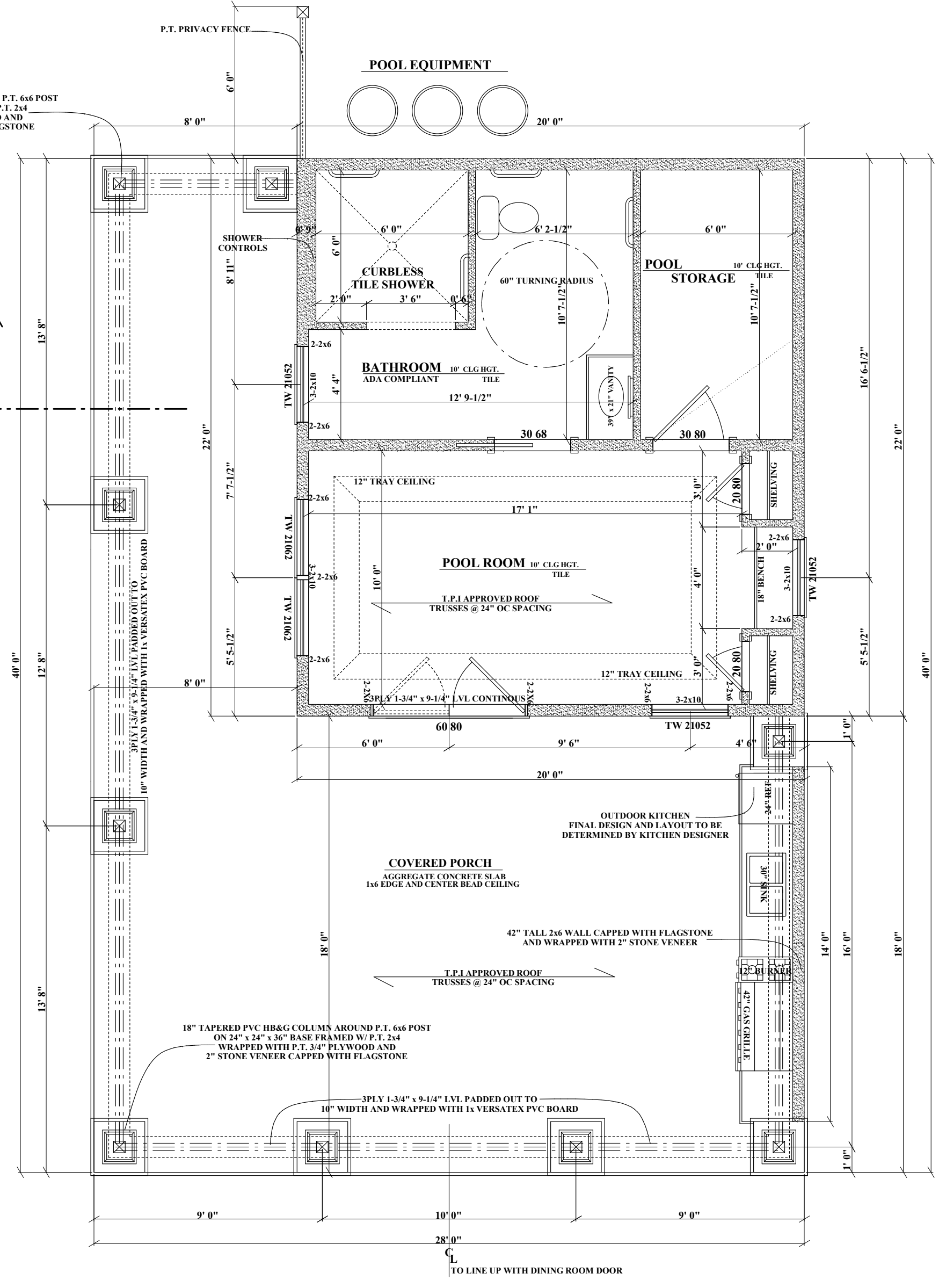
FLOOR PLAN
