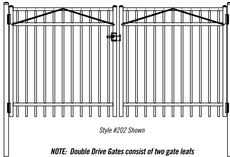
DOUBLE SWING DIMENSIONAL DRAWING
