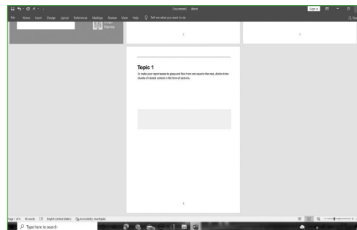
Fig. 5.20 : Topics / Sections
