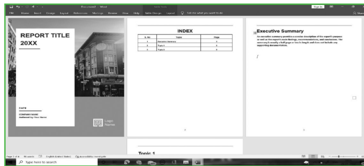
Fig. 5.19 : Executive Summary
