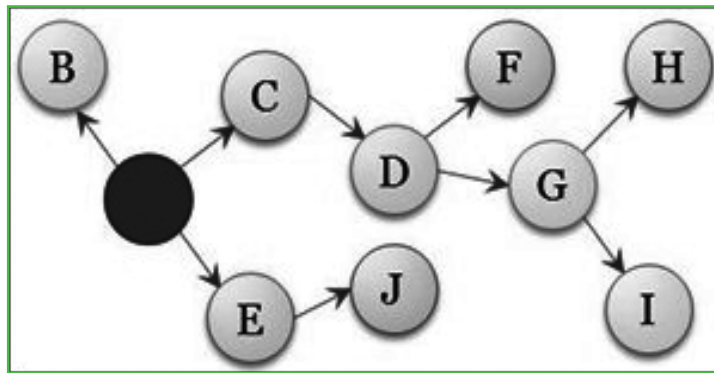
Fig. 5.6 : Probability Chain
