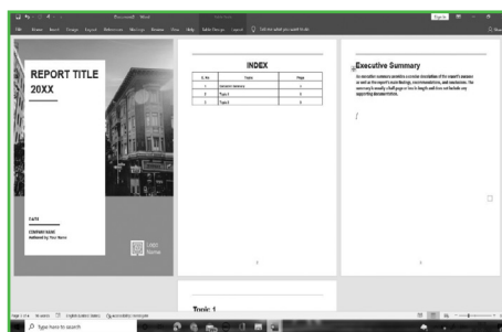
Fig. 5.17 : Cover Page
