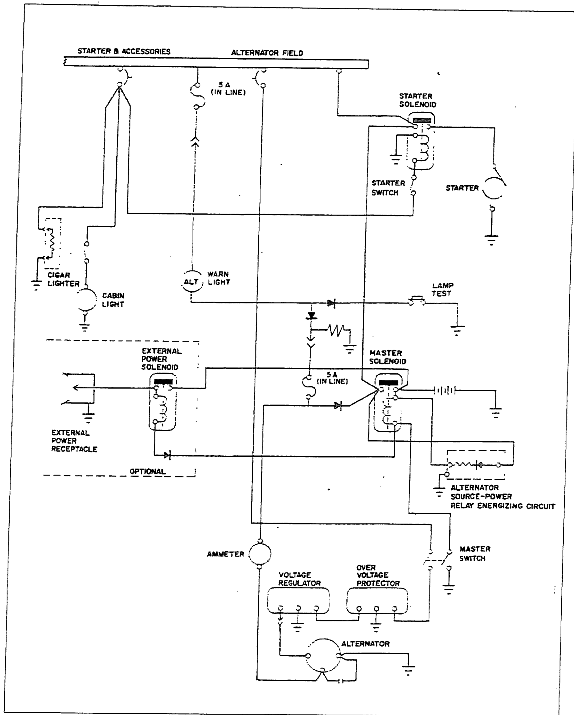
Alternator and Starter Schematic (Ser. nos. 7505001 and up)
