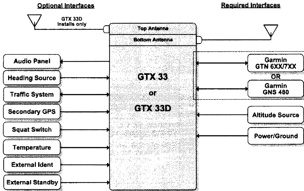
Figure 2 – GTX 33 or GTX 33D Interface Summary
