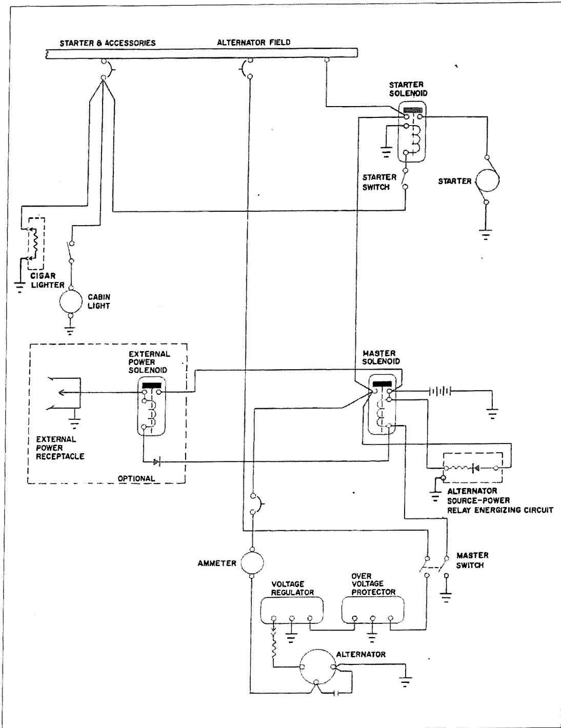
Alternator and Starter Schematic (Ser. nos. 7405001 through 7405290)
