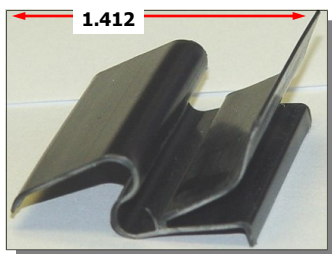
109-185 Screen clip-top
