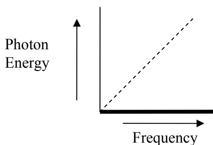
Figure 1. Direct relationship between photon energy and frequency, according to E = hv .
