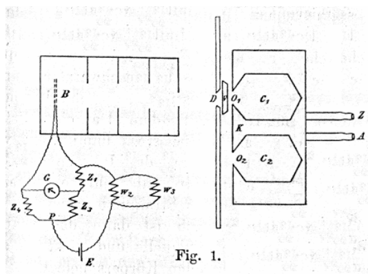
Figure 4. Schematic of the black-body device used by Ferdinand Kurlbaum at the PTR, to make black-body measurements. In 1898 Kurlbaum found that the black-body radiation from the chamber at 100^\circ\text{C} was 0.0731\text{ watts/cm}^2 more, than when the chamber was at 0^\circ\text{C} .
