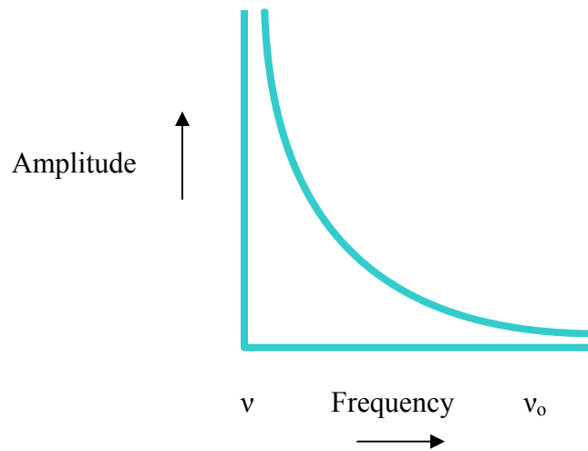
Figure 2. Amplitude plotted as a function of an applied resonant force. As the outside frequency “ v_0 ” approaches the resonant frequency “ v ”, the amplitude of the system’s oscillations increases dramatically.
