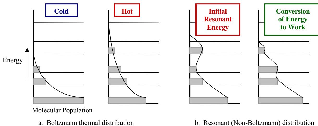
Figure 4. Diagrammatic comparison of Boltzmann energy state distribution to Resonant energy state distribution. The vertical axis represents increasing energy states, and the horizontal axis represents the number of molecules populating a particular energy state.
