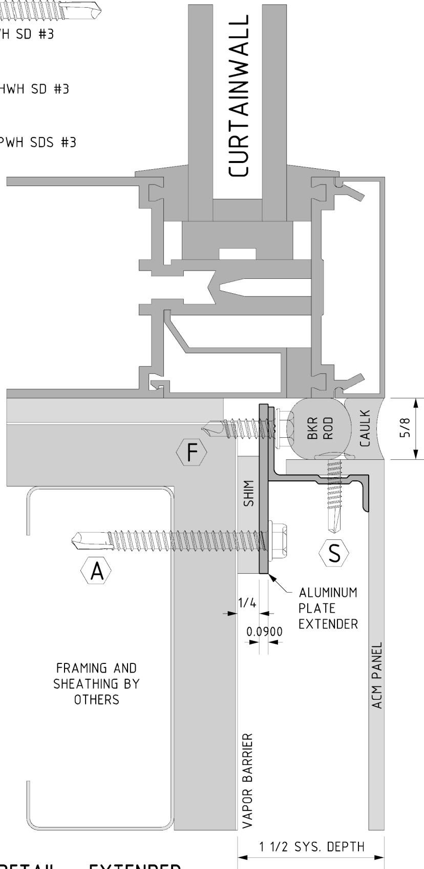
SILL TERMINATION DETAIL - EXTENDER
