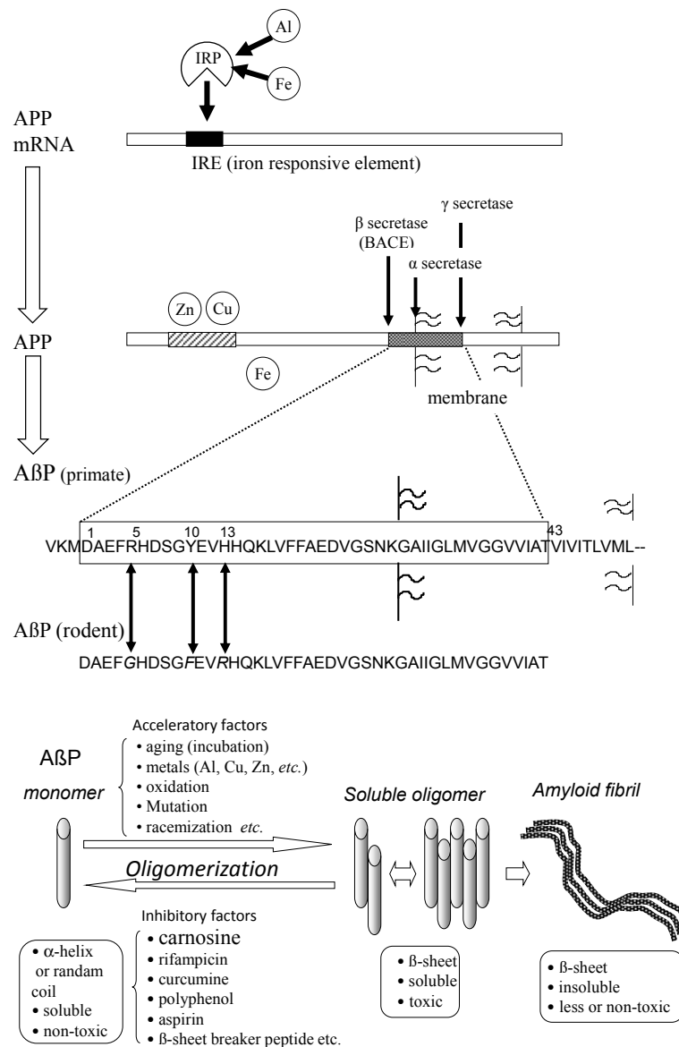
Figure 4. Secretion and oligomerization of A \beta P. A \beta P is secreted from APP by \beta -secretase (BACE) and by \gamma -secretase. The expression of APP is regulated by Fe and may be influenced by Al. APP also binds to Cu and Zn. Three amino acids (Arg 5 , Tyr 10 , and His 13 ) of human A \beta P are substituted in rodent A \beta P. Under aging conditions or in the presence of acceleratory factors, monomeric A \beta P with random or \alpha -helix structures self-aggregates and forms several types of oligomers (SDS-soluble oligomers, amyloid \beta -derived diffusible ligands, globulomers, protofibrils) before finally forming insoluble aggregates (amyloid fibrils). The monomeric and fibril aggregates are relatively nontoxic; however, oligomeric soluble A \beta Ps are toxic. APP: amyloid precursor protein; mRNA: messenger ribonucleic acid; A \beta P: \beta -amyloid protein; Al: aluminum; Fe: iron; IRP: iron regulatory protein.
