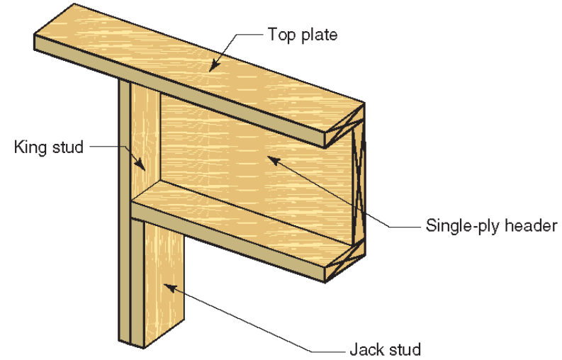
Components of an alternative single member header
