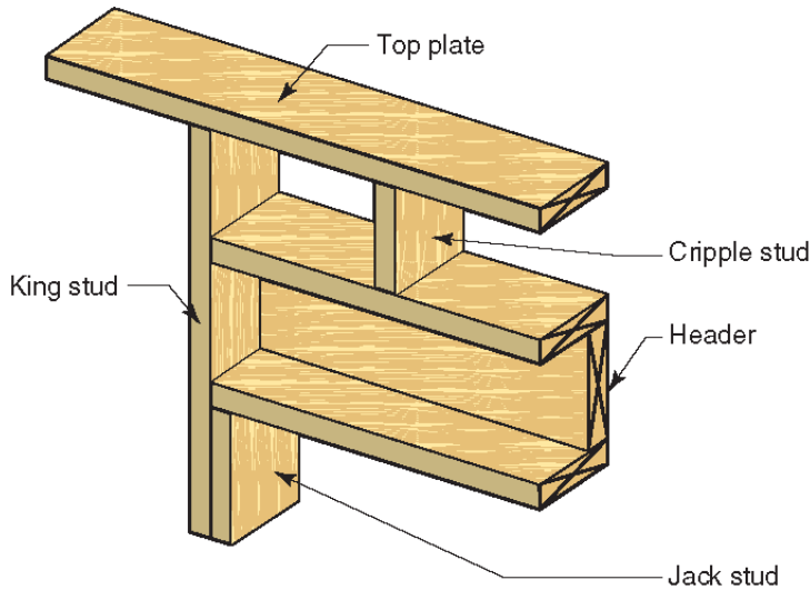
Components of a single member header
