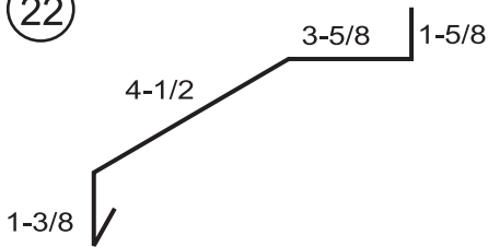
Top Mount Track Cover
