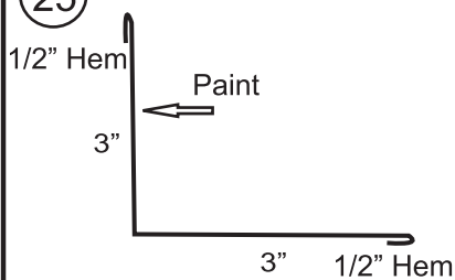
Inside Angle
