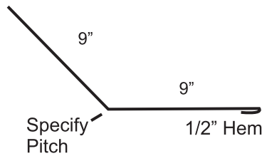
Transition Flashing
