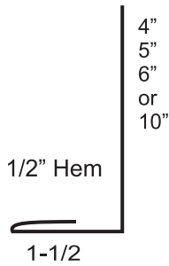
Fascia
