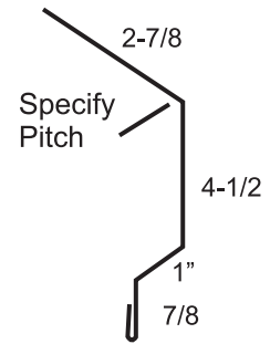
Fascia Eave
