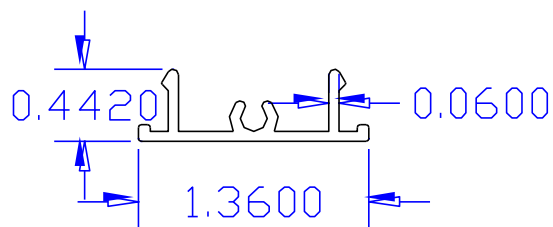
CLIP VERTICAL-HORIZONTAL
