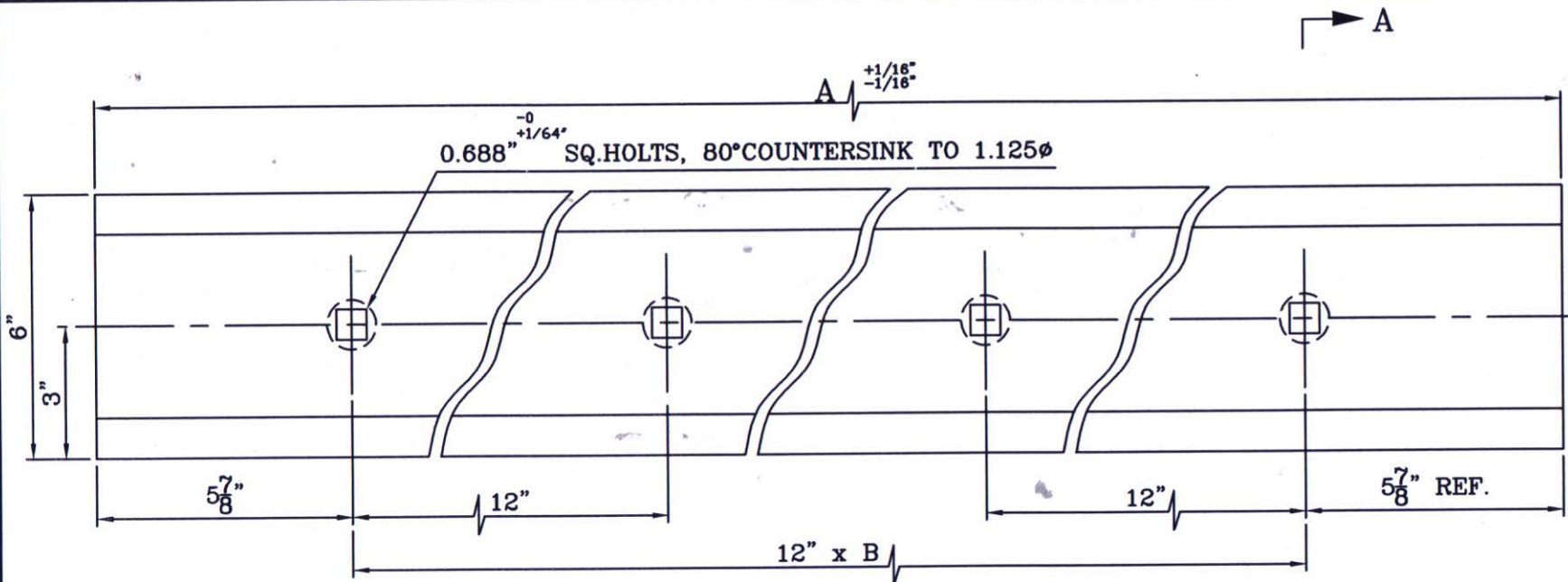
FRONT ELEVATION
