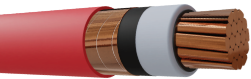
3 Cable N2XSY
