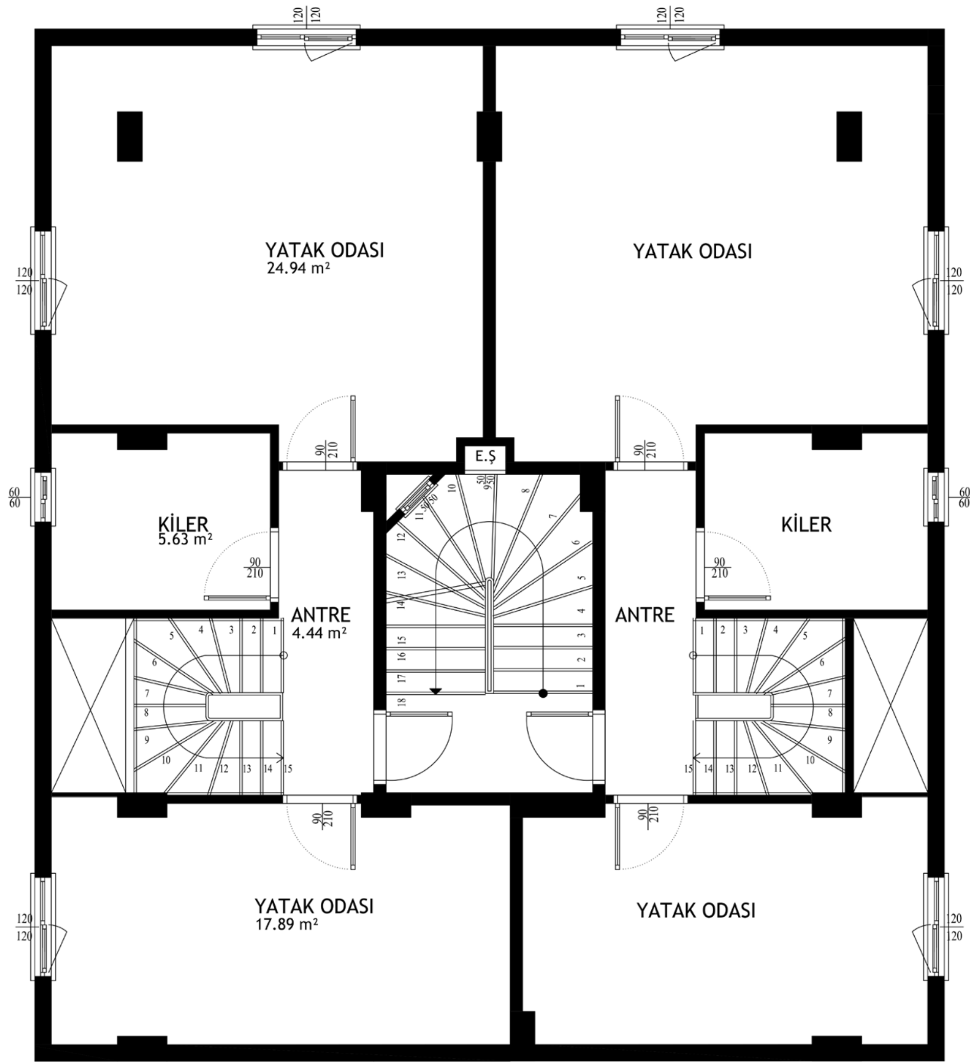
BODRUM KAT PLANI
