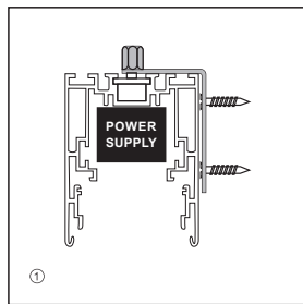
① 安装型材至墙壁 Installing profiles to wall
