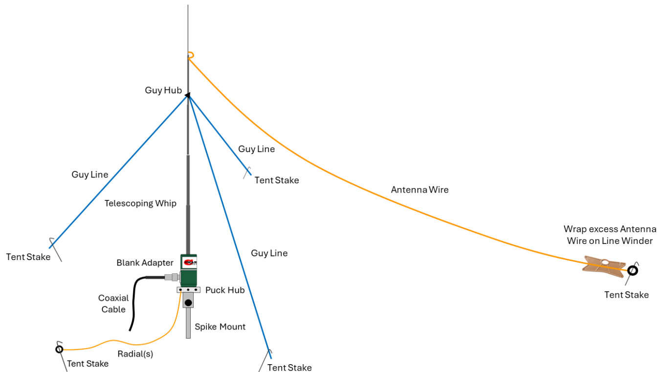
Figure 3. CHA BV 60, 75, and 80 Meter Inverted Lazy “L” Antenna.
