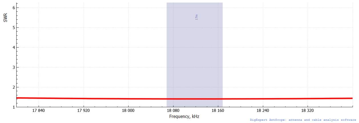
Figure 8. 17 Meter SWR Graph.
