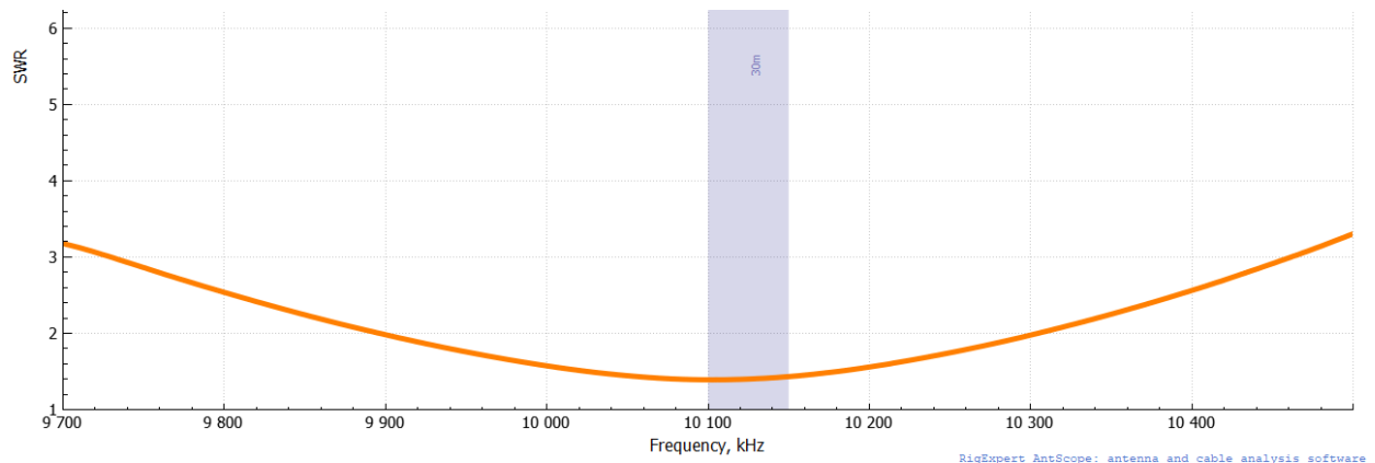
Figure 6. 30 Meter SWR Graph.
