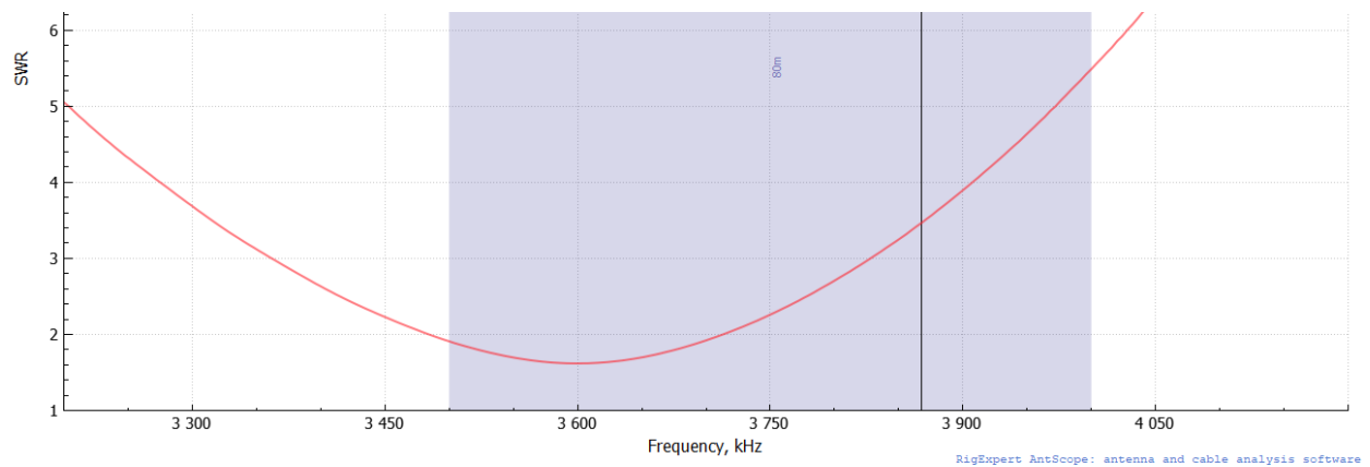
Figure 11. 80 Meter Inverted Lazy "L" SWR Graph.
