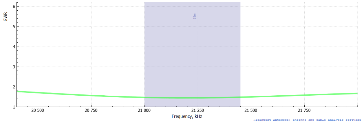
Figure 9. 15 Meter SWR Graph.
