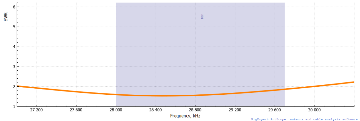
Figure 11. 10 Meter SWR Graph.
