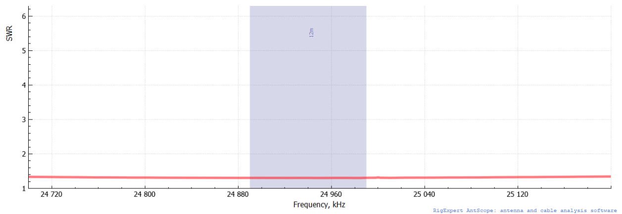
Figure 10. 12 Meter SWR Graph.
