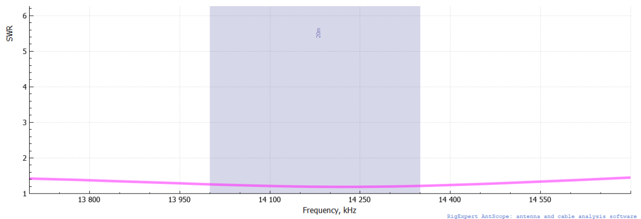
Figure 7. 20 Meter SWR Graph.
