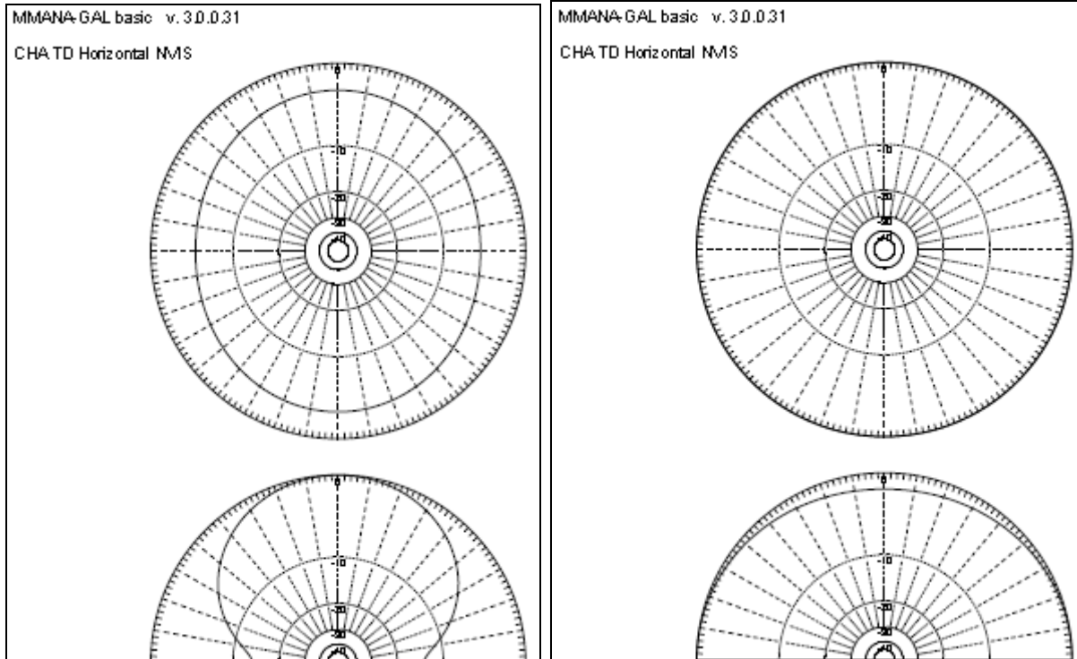
Figure 9. Horizontal NVIS Far Field Plots, 3.7 (left) and 7 (right) MHz.
