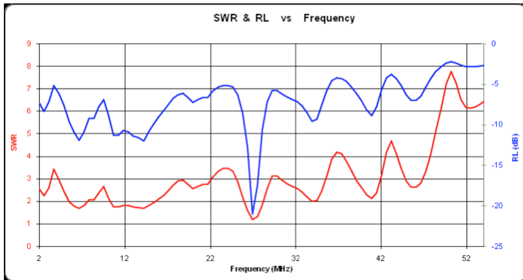
Figure 6. SWR vs Frequency Graph.
