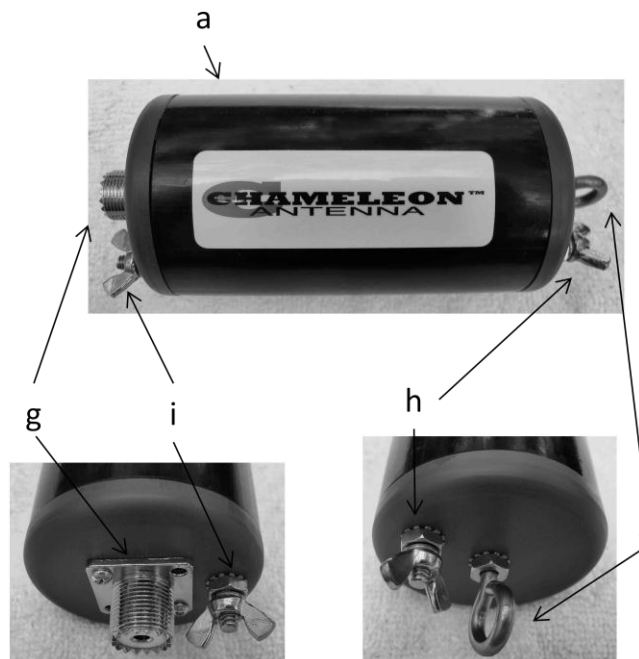
Plate 1. Matching Transformer, Side View (top), Bottom View (left) and Top View (right).
