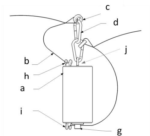
Figure 2. Matching Transformer Electrical and Mechanical Connections.
