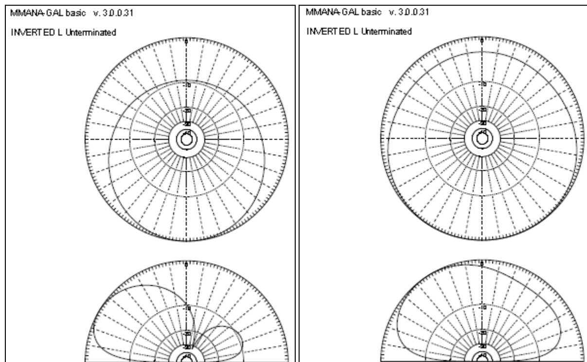
Figure 8 Inverted "L" Far Field Plots, 3.7 (left) and 7 (right) MHz.
