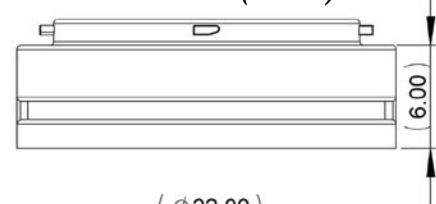
RB-R-22x6 (Riser)
