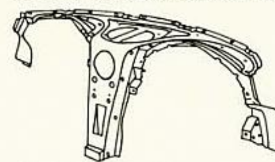
Instrument panel construction
