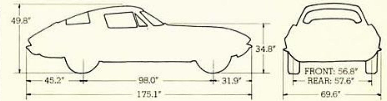
External dimensions, Sport Coupe
