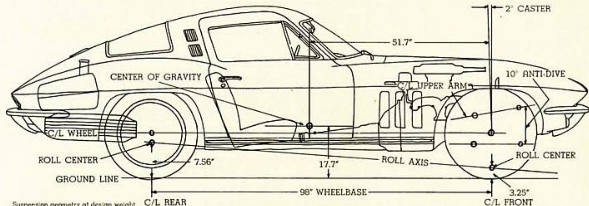
Suspension geometry at design weight
