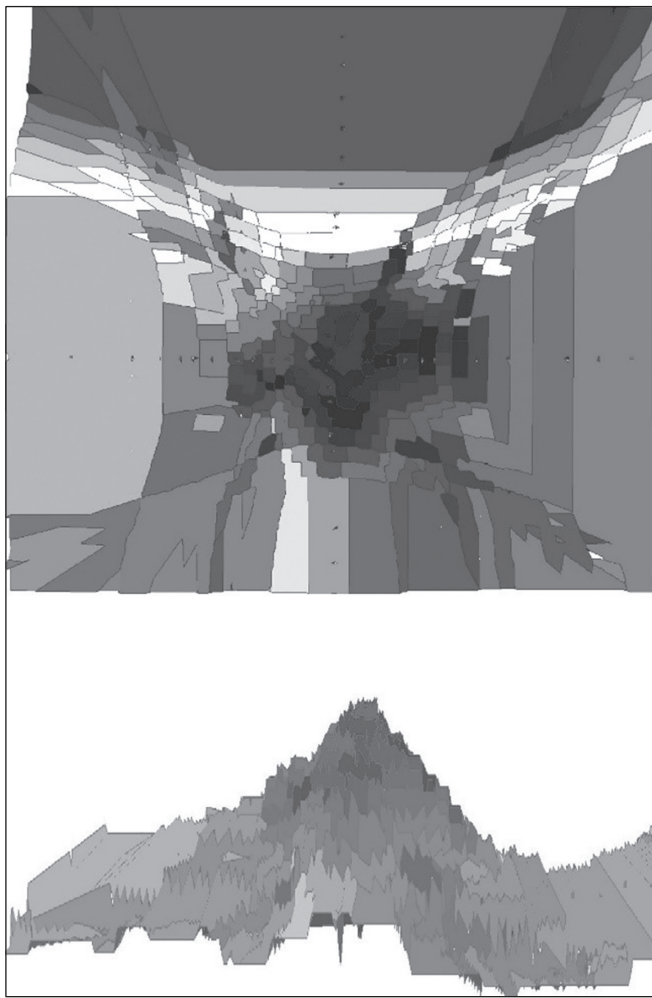
Figure 5. Both 2-D and 3-D renderings of the magnetic susceptibility signal from the hearth feature. The upper vertical 2-D image depicts the focus of the hearth and the lower 3-D oblique image depicts the relative magnitude of the fire-induced magnetic signal. Horizontal dimension of the image is 90 cm.
