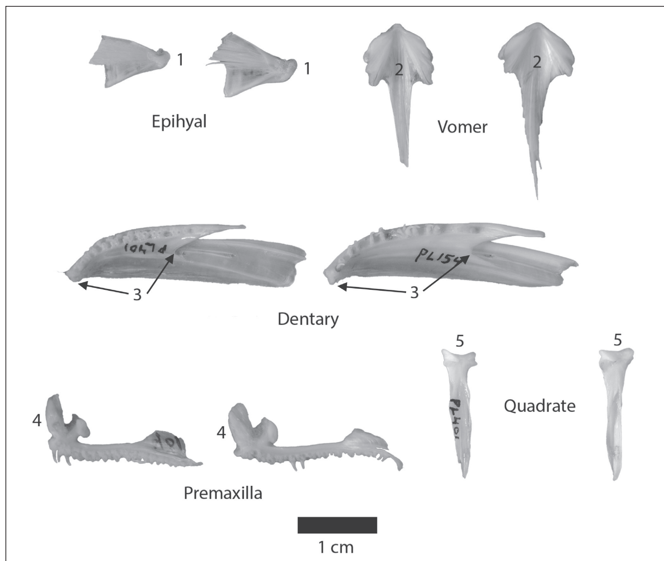
Figure 3. Pairs of the five elements from a comparative saffron cod (left of each pair) and Pacific cod (right), each showing an example distinguishing characteristic. Epihyal: the posterior process (1) is narrower in saffron cod. Vomer: the dorsal (nontoothed surface) has a narrower upside-down V-shaped cleft (2) in saffron cod. Dentary: the anterior-posterior diameter from the symphysis to the interior-posterior incision (3) is shorter in saffron cod. Premaxilla: the ascending process (4) is narrower and taller in saffron cod. Quadrate: the articulation (5) is more concave in saffron cod. All elements shown are right side. Saffron cod elements from specimen PL-401 (total length 35 cm) and Pacific cod elements from PL-154 (total length 30 cm).
