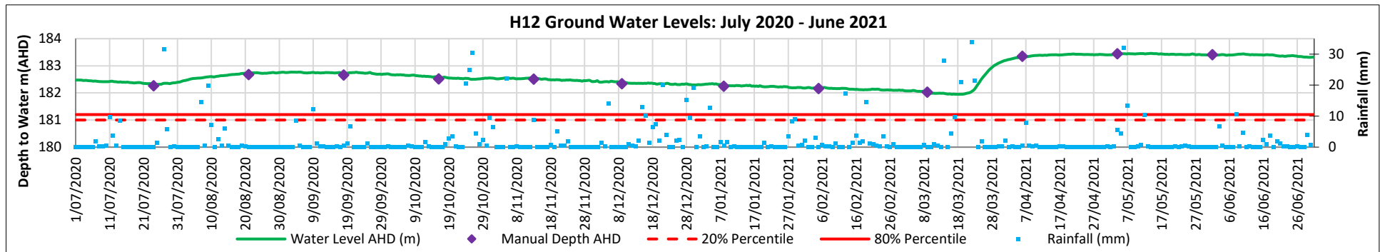
Chart 24: H12 Groundwater Levels for July 2020 – June 2021
