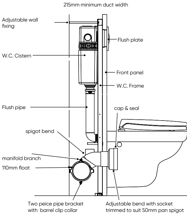
Manifold branch
