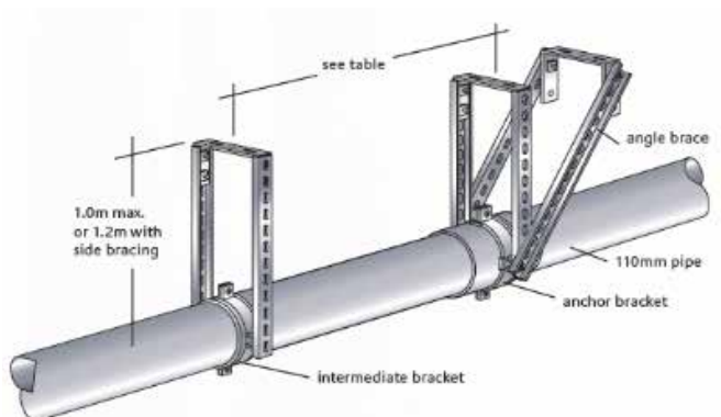
Double support
