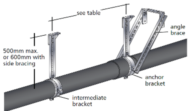
Single support
