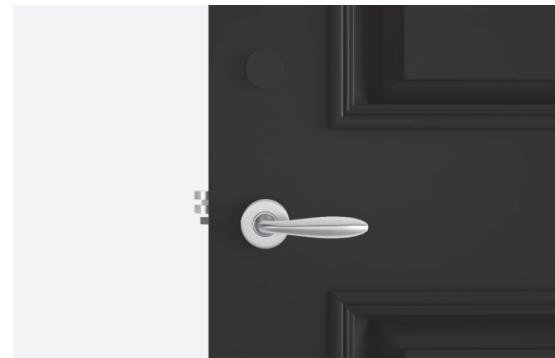
7: Mach
