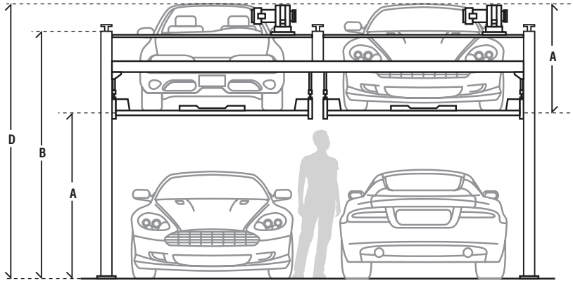
Typical dimensioning for the CARLOFT. Dimension can be modified to fit the garage design This is based on one car above and one car at grade. *Average vehicle length is 16' 6".
