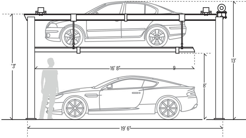
Typical dimensioning for the CARLOFT. Dimension can be modified to fit the garage design This is based on one car above and one car at grade. *Average vehicle length is 16' 6".
