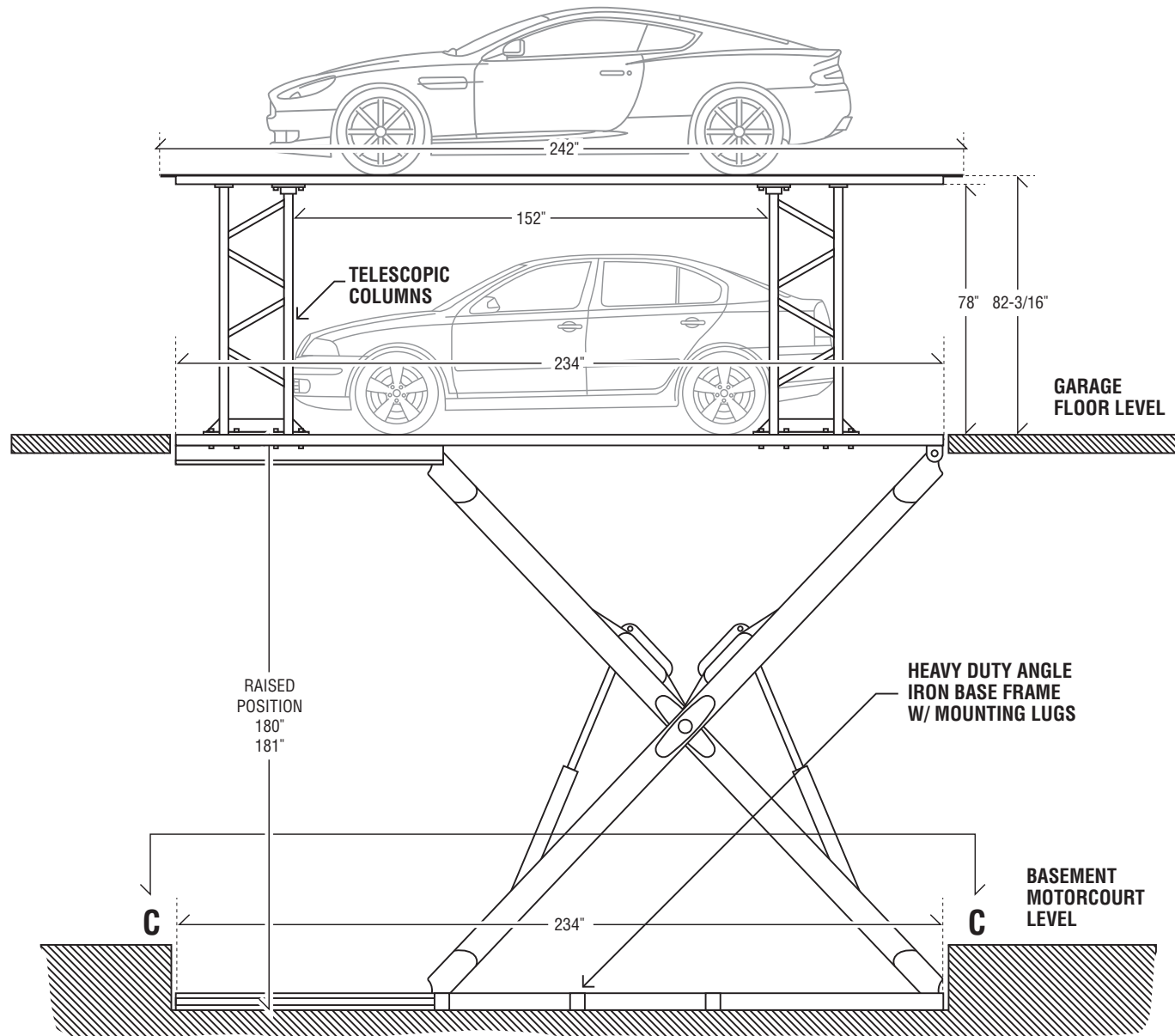
FIG. 13 RAISED POSITION
