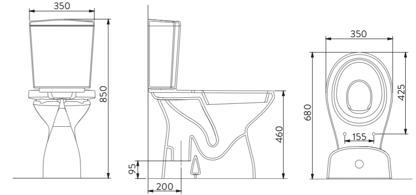
A051091H WC PAN | WITHOUT BIDET FUNCTION
