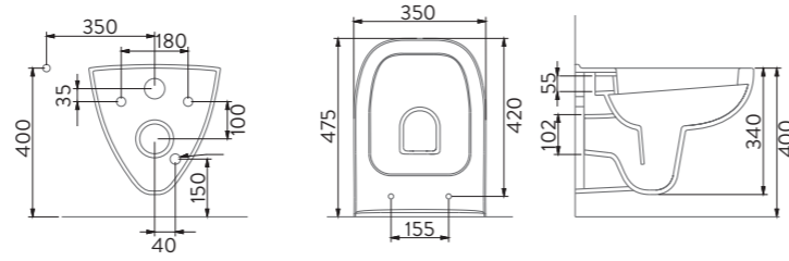
PETITE RIM - OUT ASMA KLOZET PETITE RIM - OUT WALL-HUNG WC PAN
