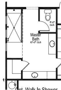
Opt. Walk In Shower at Master Bath
