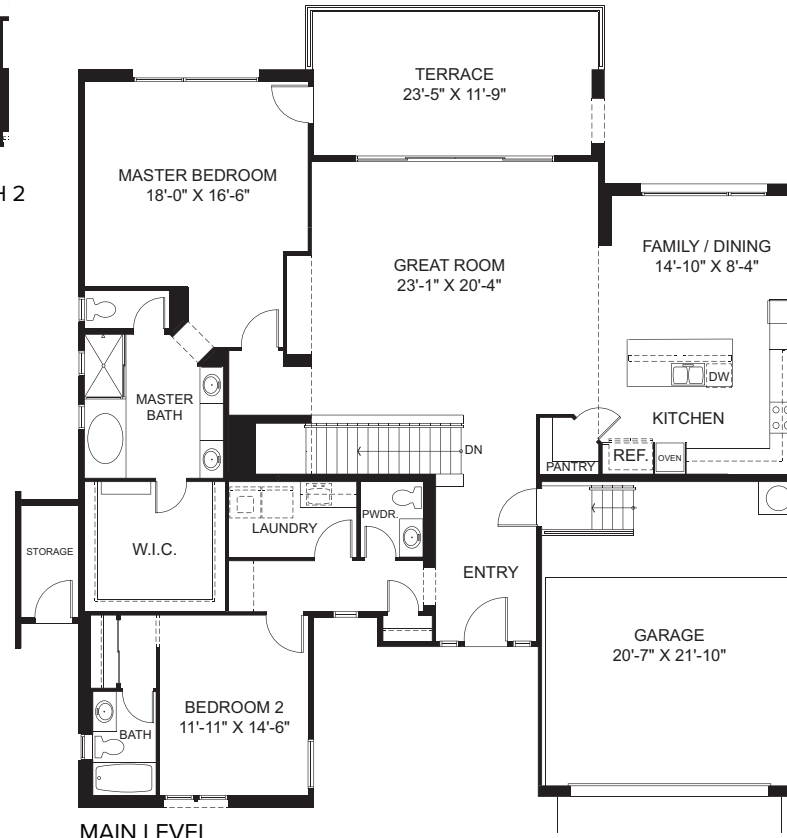
MAIN LEVEL
