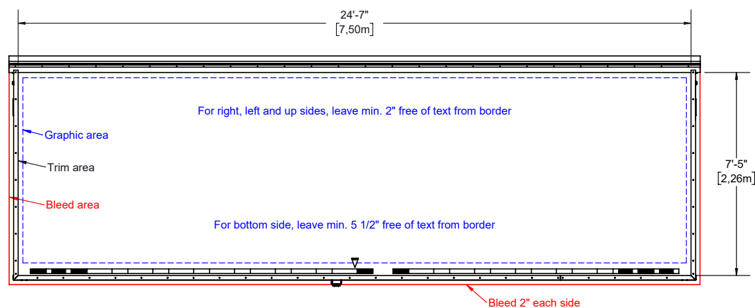
SIDE PANEL SCALE 1:50 QTY. 2
