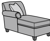
5990-25 LAF Chaise 36H 33W 62D 21SH 25SW 49SD 27AH
