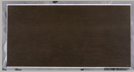
Java #10
