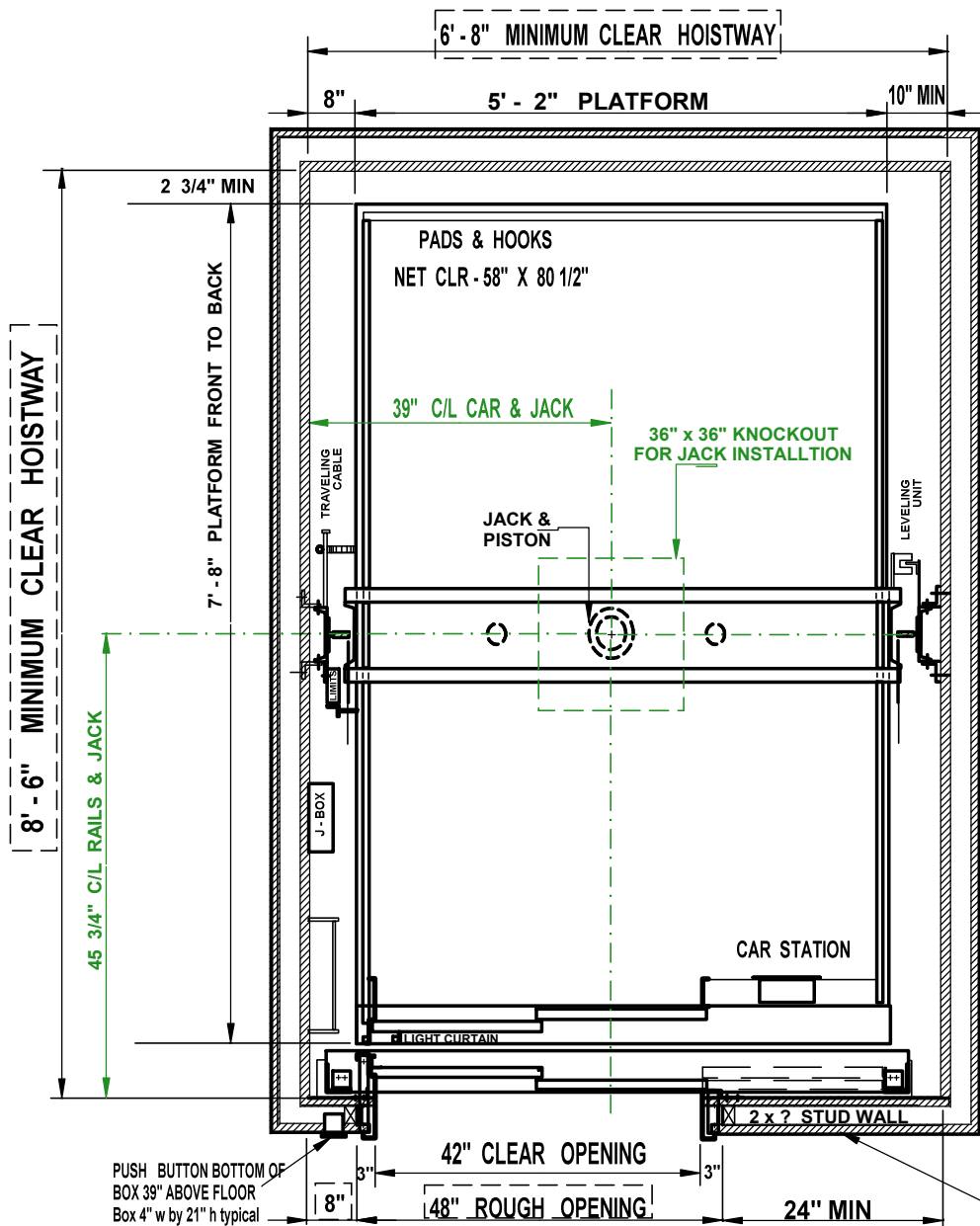
PLAN VIEW - HOISTWAY WOOD LEVELS
