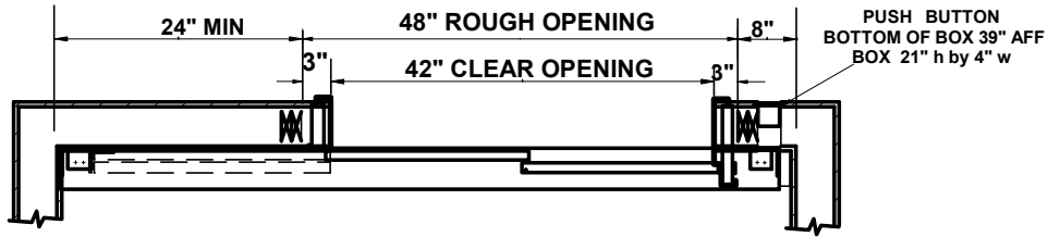
PLAN VIEW - ENTRANCES WOOD LEVELS
