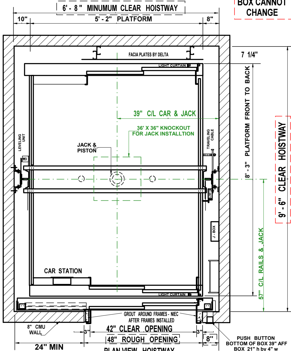
PLAN VIEW - HOISTWAY CONCRETE LEVELS
