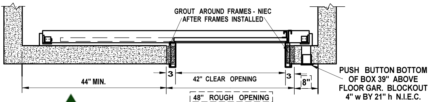
PLAN VIEW OF BLOCK/CONCRETE ENTRANCE
