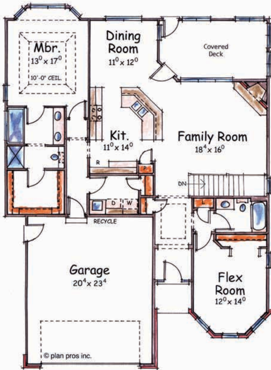
FLOOR PLAN
