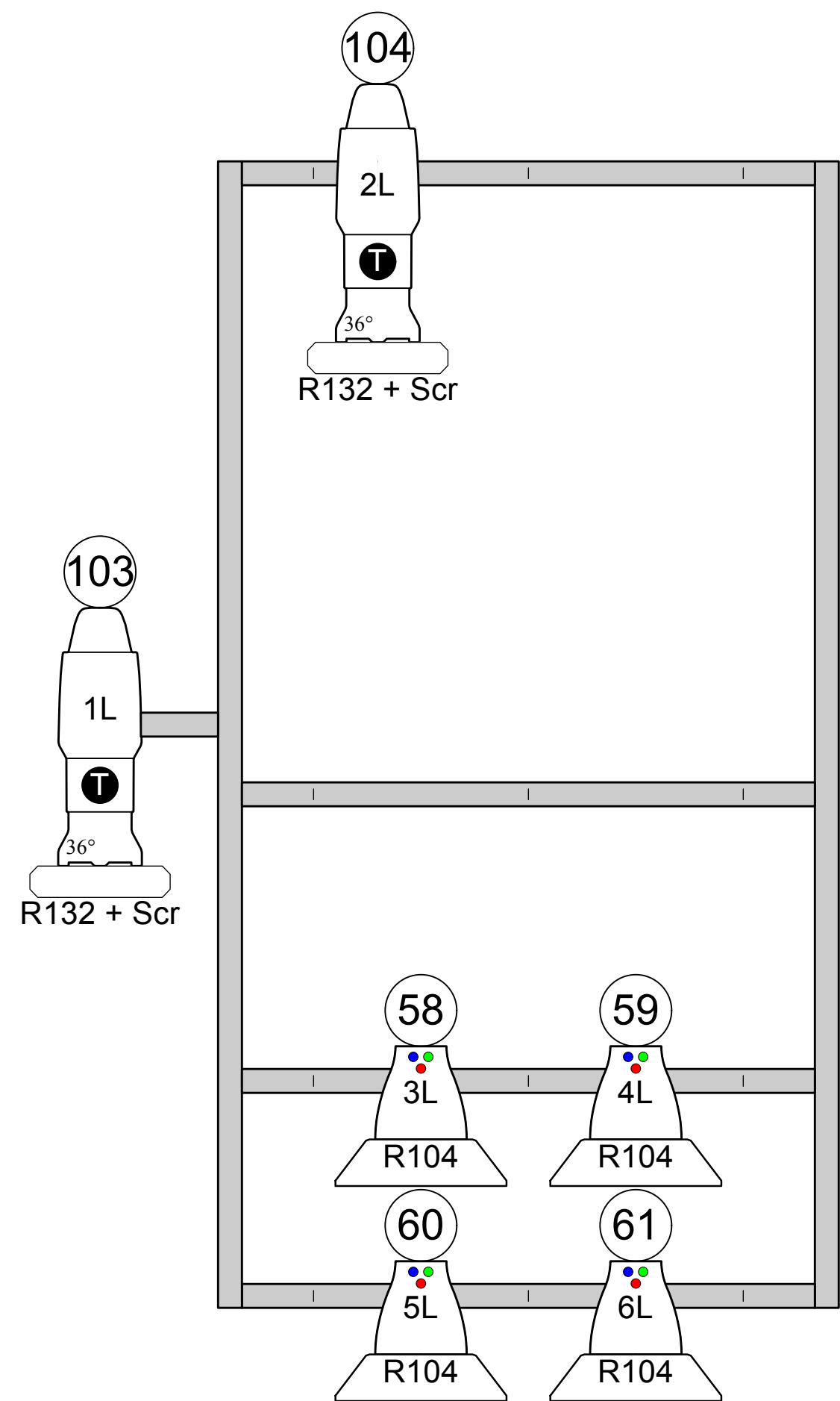
FOH Left Ladder
