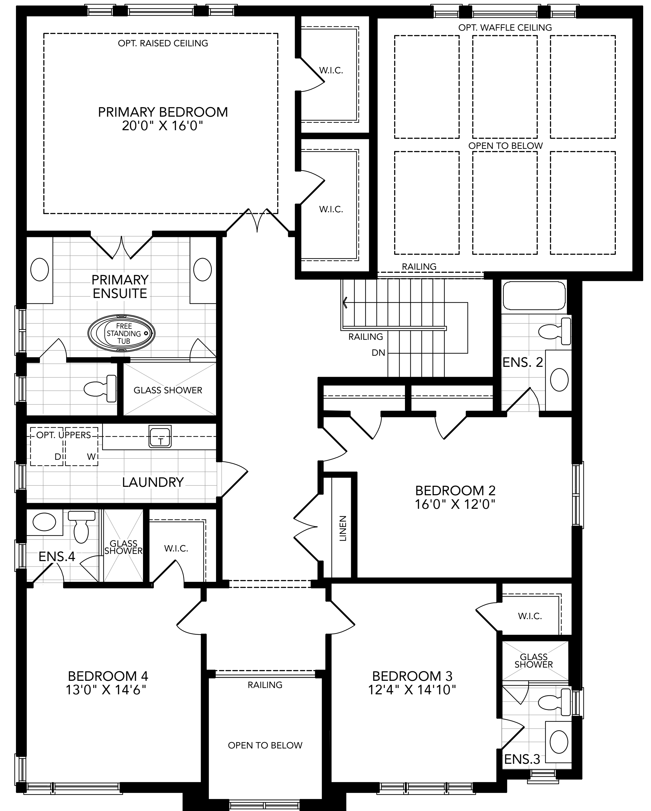
Second Floor Plan Elevation B
